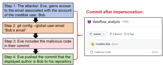
Fig. 2. A motivating example showing impersonation of a legitimate user.
